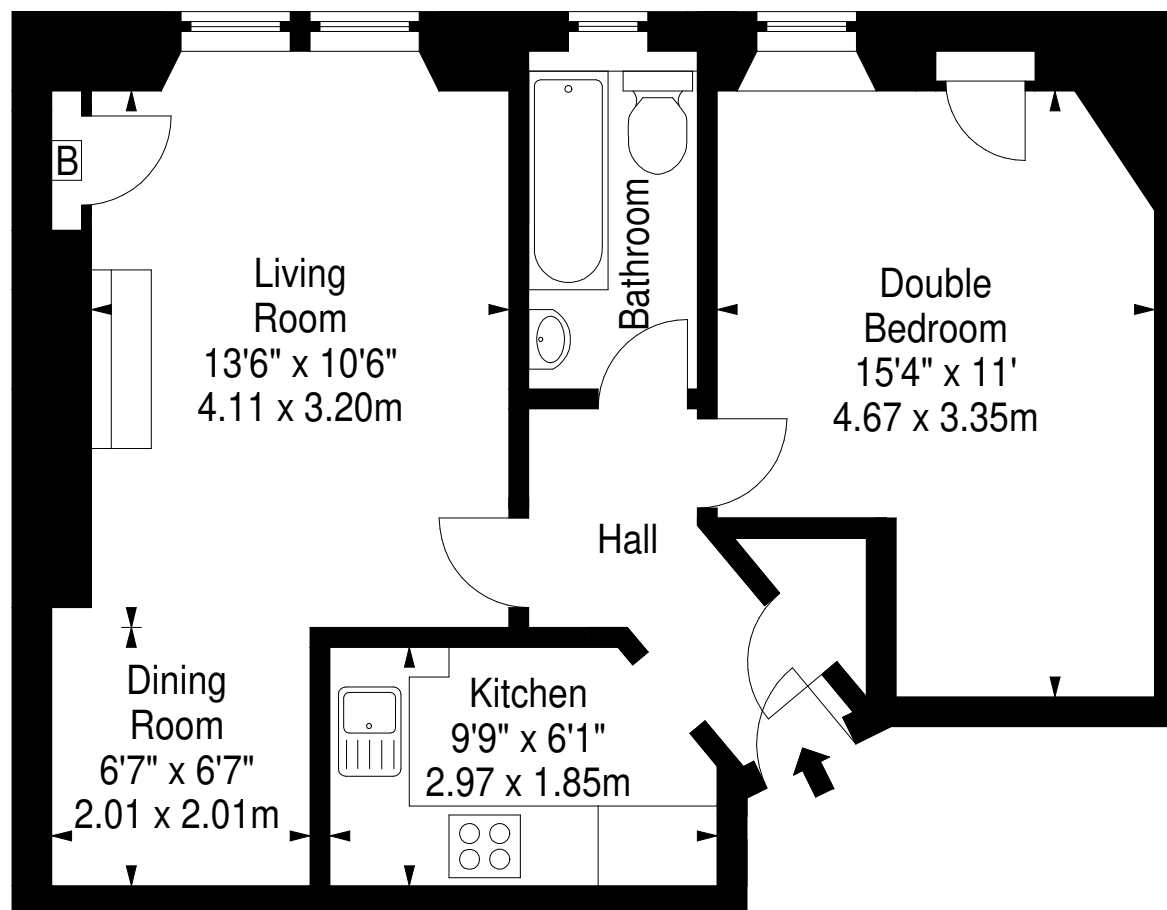
First Floor
