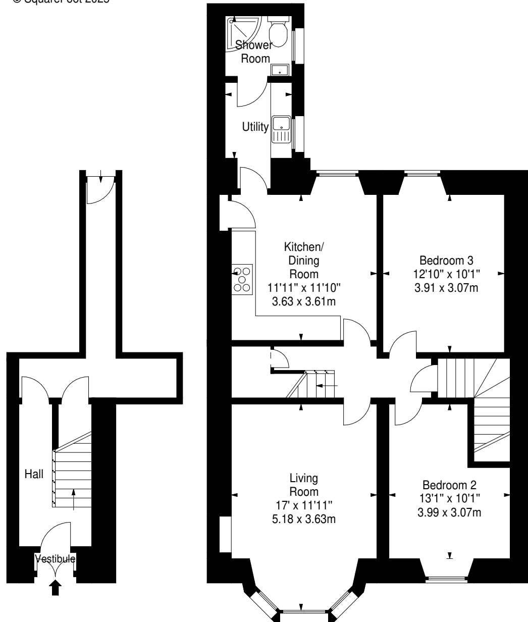
Ground Floor
