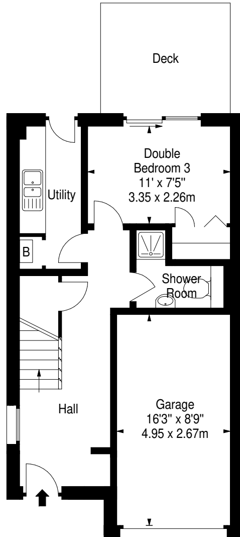
Ground Floor
